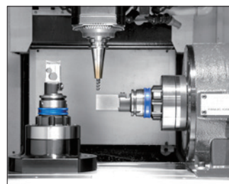
Multi-face machining with single 3-axis machine
