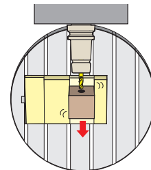
Insufficient clamping strength in machining direction
